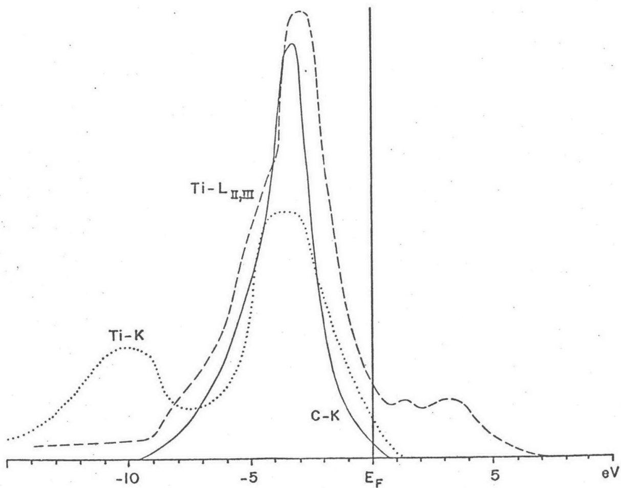
FIG. 8. TiC soft x-ray emission.
